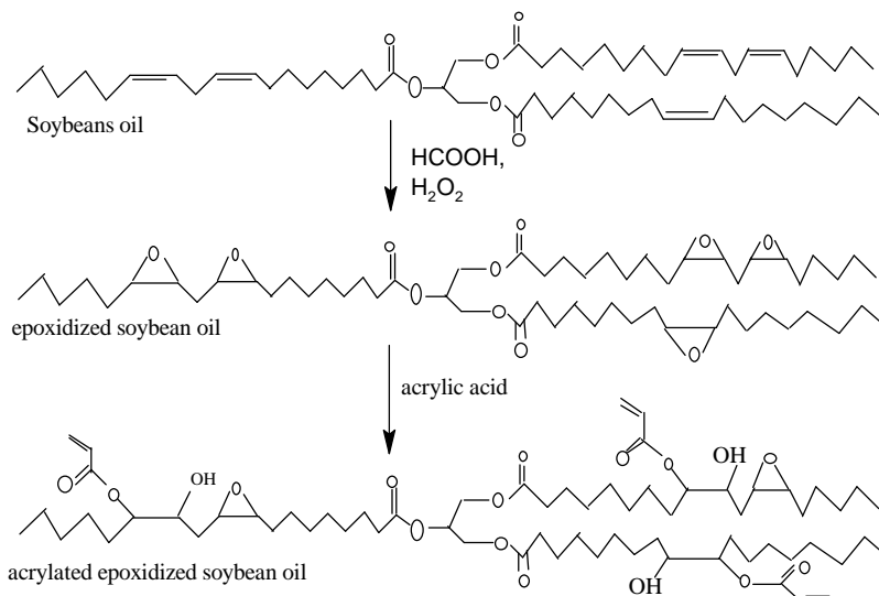
Figure 2. Synthesis of acrylatedepoxidised soybean oil [31].
