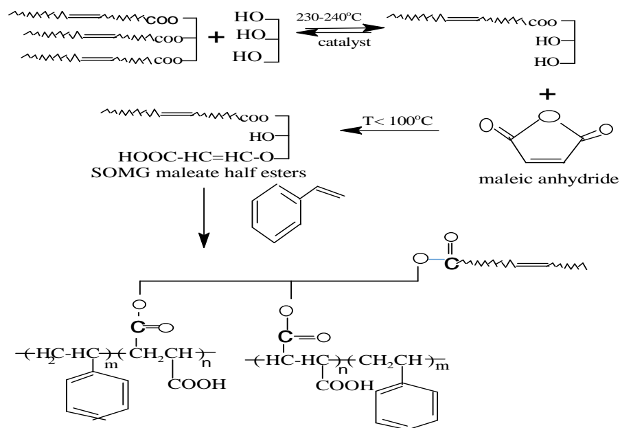
Figure 3. Synthesis and polymerization of soybean oil monoglyceride maleates [32].
